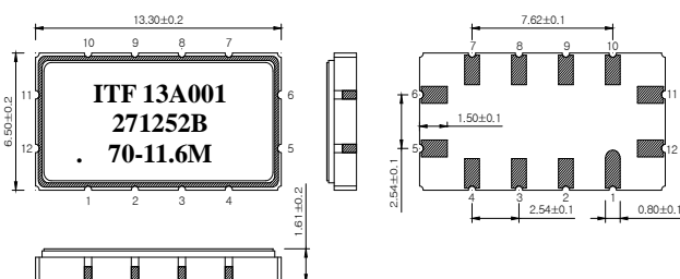
S1365 Package Dimension
