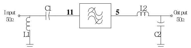
Matching Schematic
