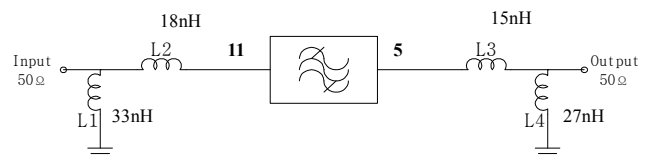
Matching Schematic
