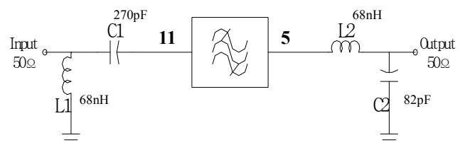
Matching Schematic
