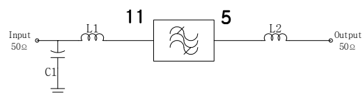
Matching Schematic
