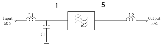
Matching Schematic
