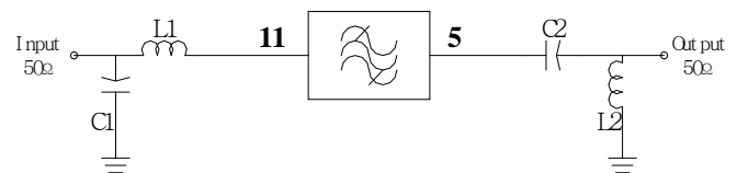
Matching Schematic
