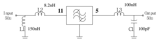
Matching Schematic
