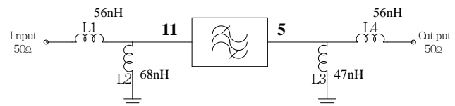
Matching Schematic
