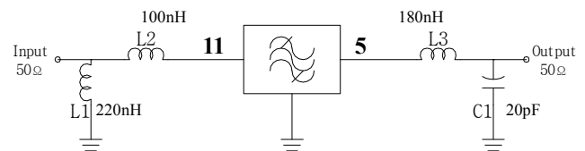
Matching Schematic
